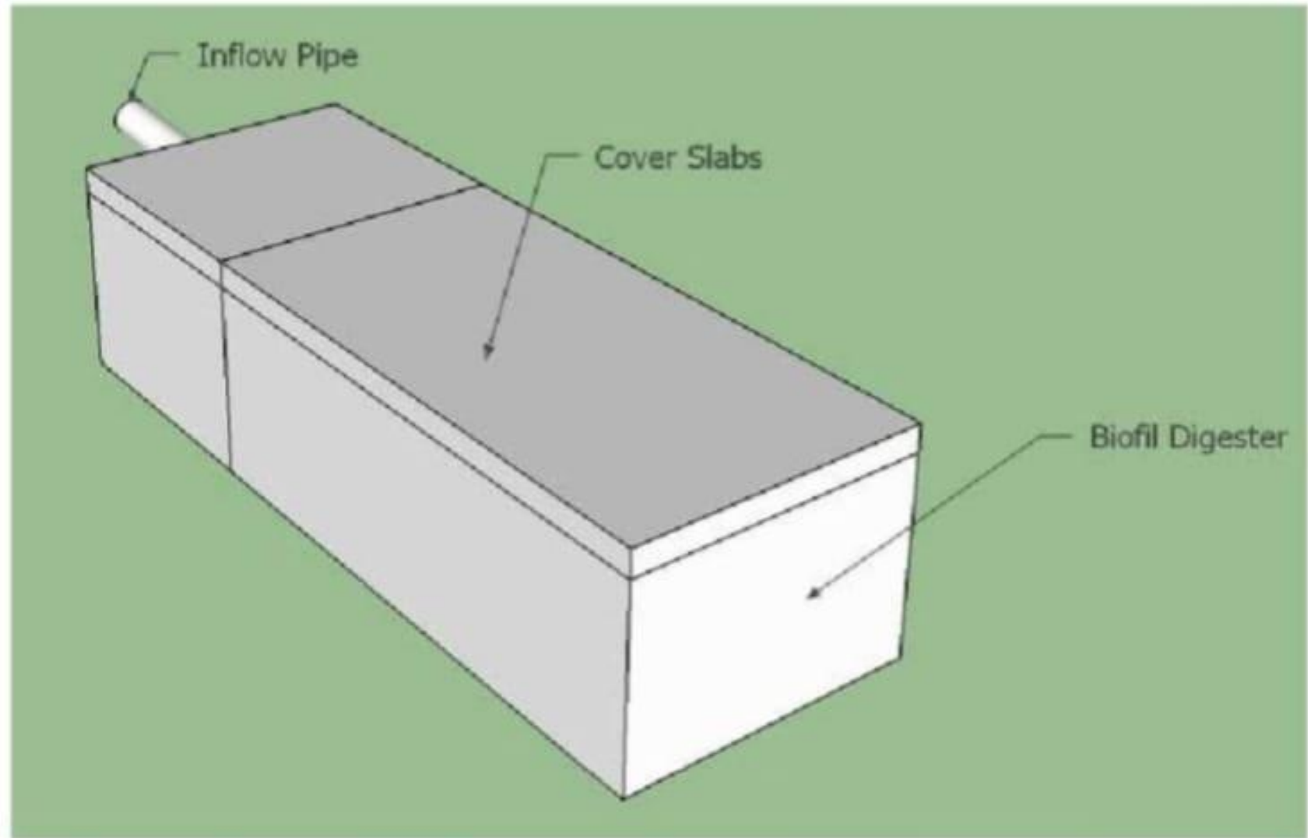
Fig. 1: Schematic View (Outer) of the Biofil Digester
